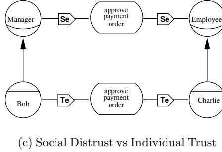
Fig. 3. Conflicts on (dis)trust relations
