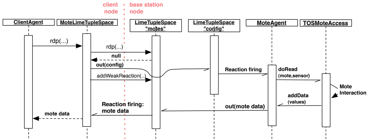
Fig. 10. Sequence diagram showing the processing of a rdp.
