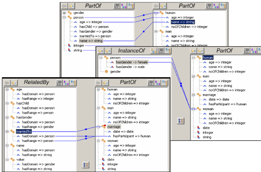
Figure 6-6 Mapping views in the AML View-Based Editor.
