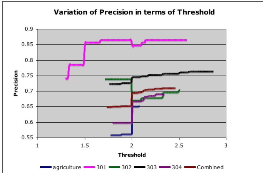
Fig. 1. Precision variation in terms of threshold values set for the length of the derivation path.
