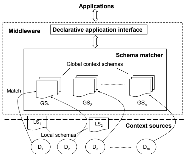
Figure 1. Schema matching in context-aware middleware
