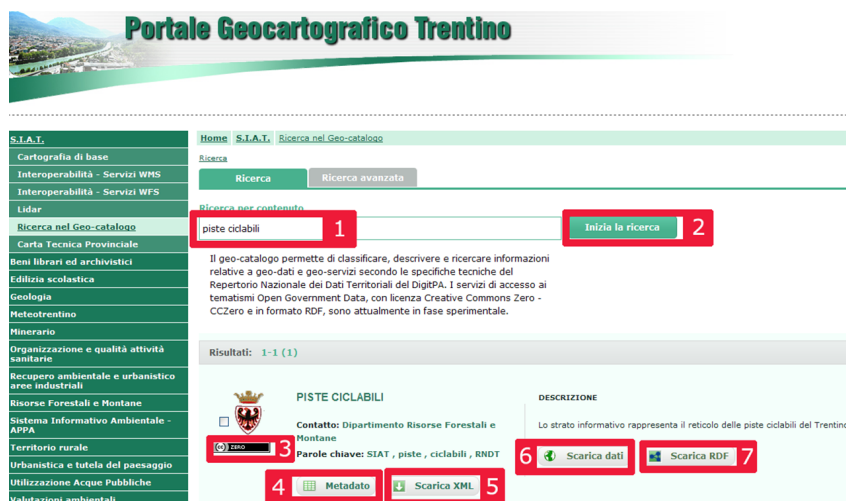
Fig. 5: Search results.
