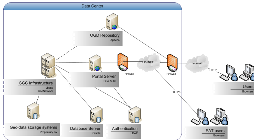
Fig. 4: System architecture.
