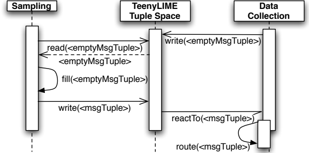
Figure 6: Handling sampled data over for routing.
